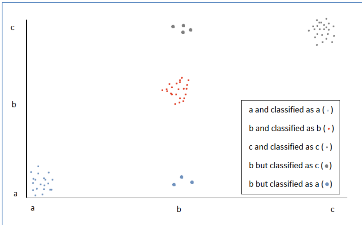
Figure 6. Classification errors of TAN Algorithm
