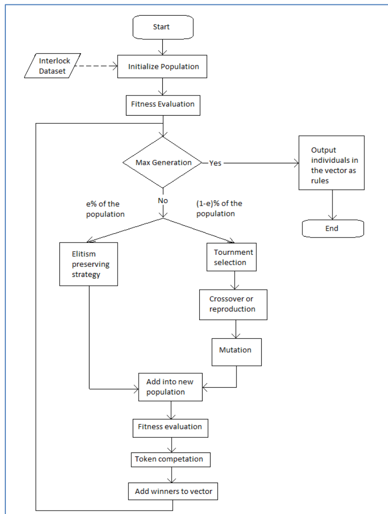
Figure 3. Flow diagram of the TAN algorithm used
