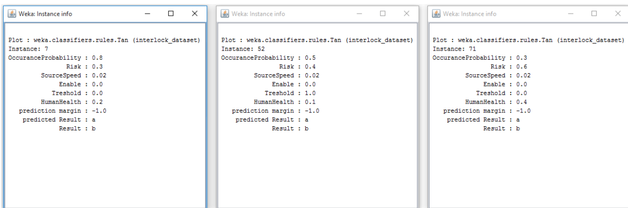
Figure 7. Classification information for instances that can not be classified correctly (instances classified as 'a' when it should be classified as 'b')
