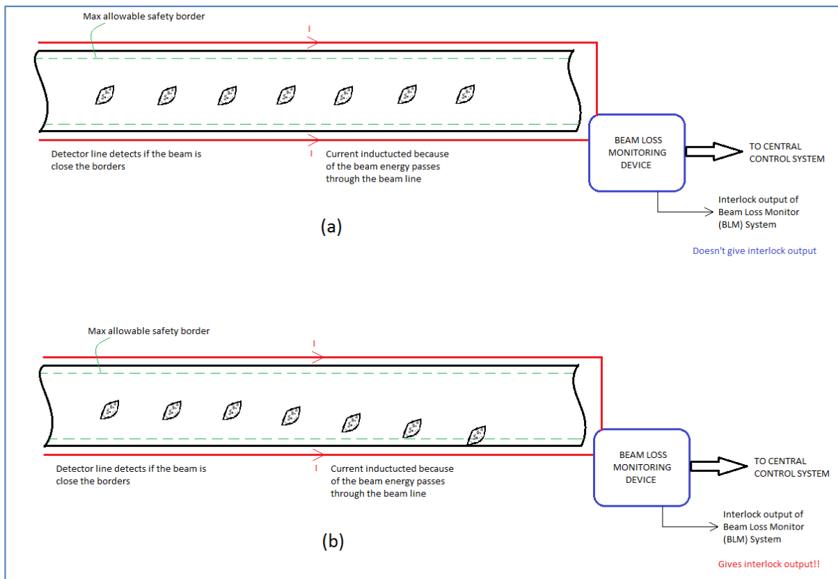
Figure 2. Basic layout of the Beam Loss Monitoring (BLM) system as example of an interlock source
