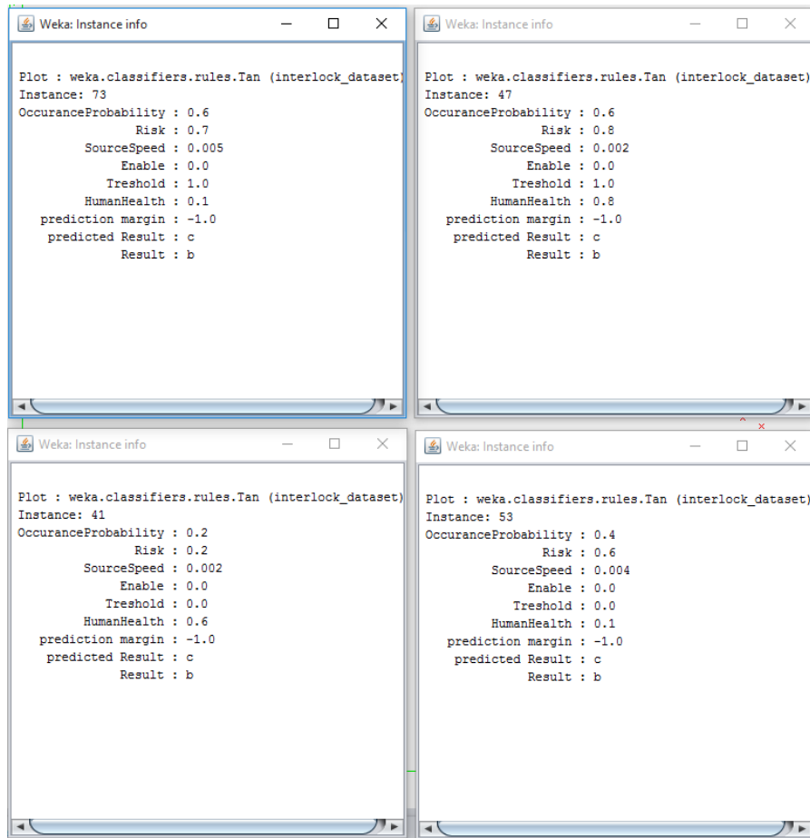
Figure 8. Classification information for instances that can not be classified correctly (instances classified as 'c' when it should be classified as 'b')
